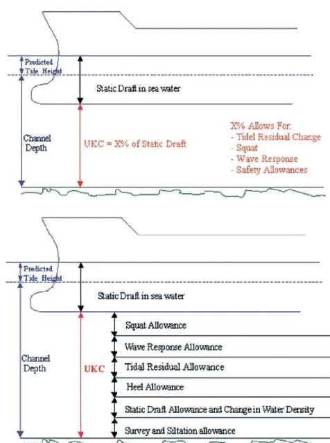
Figure 34 - Vessel Under Keel Clearance (UKC)
